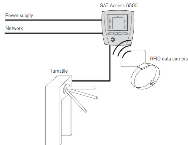
Typical application
